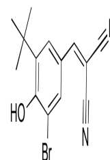
Chemical structure of AG-1024
