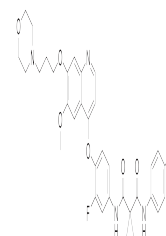
Chemical structure of Foretinib
