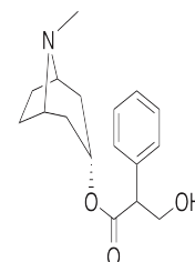
Chemical structure of Atropine
