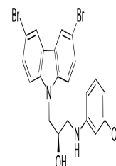
Chemical structure of (R)-P7C3-OMe
