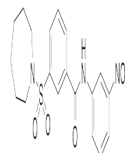
Chemical structure of AK-1
