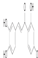
Chemical structure of Butein
