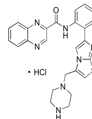
Chemical structure of SRT1720 Hydrochlor...
