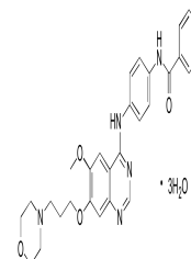
Chemical structure of ZM-447439 Trihydrate...
