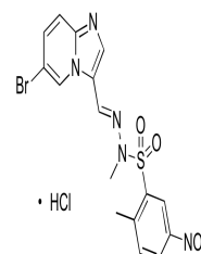
Chemical structure of PIK-75 Hydrochloride...
