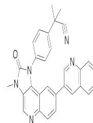
Chemical structure of BEZ235
