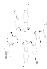
Chemical structure of TL-32711
