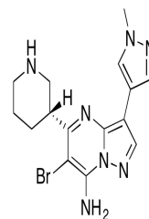
Chemical structure of SCH-900776
