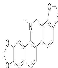
Chemical structure of Dihydrosanguinarin...
