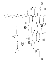
Chemical structure of Caspofungin Diacet...
