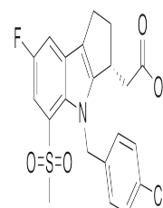
Chemical structure of MK-0524
