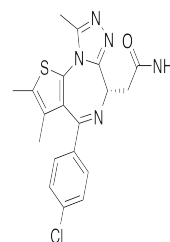
Chemical structure of CPI-203
