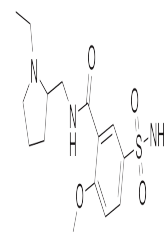
Chemical structure of R
