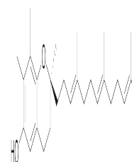
Chemical structure of Tocotrienol
