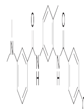
Chemical structure of ZM-336372
