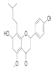
Chemical structure of Isoxanthohumol
