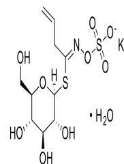
Chemical structure of Sinigrin Monohydra...
