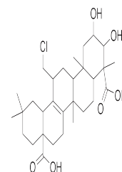
Chemical structure of Senegenin
