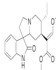
Chemical structure of Rhyncholphylline
