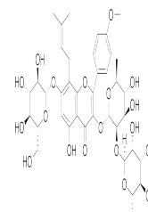
Chemical structure of Epimedin C
