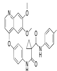
Chemical structure of Cabozantinib
