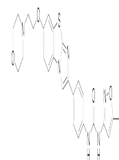
Chemical structure of Quizartinib
