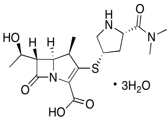
Chemical structure of Meropenem Trihydrate
