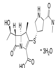
Chemical structure of Meropenem Trihydrate...
