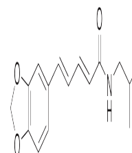
Chemical structure of Piperlonguminine
