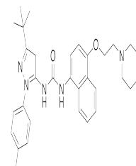
Chemical structure of Doramapimod
