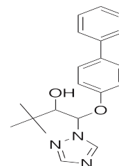
Chemical structure of Bitertanol
