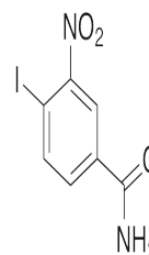
Chemical structure of Iniparib
