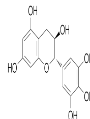
Chemical structure of (-)-Gallocatechin
