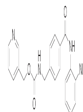
Chemical structure of Entinostat
