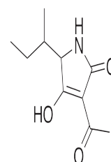
Chemical structure of Tenuazonic Acid
