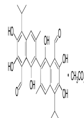
Chemical structure of Gossypol Acetic Ac...
