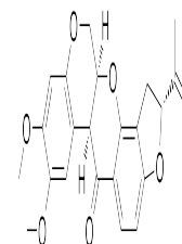
Chemical structure of Rotenone
