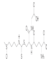
Chemical structure of S-(N-Methylsulfiny...
