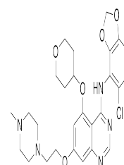
Chemical structure of Saracatinib
