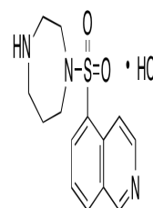
Chemical structure of Fasudil Hydrochloride...
