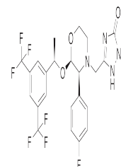
Chemical structure of Aprepitant
