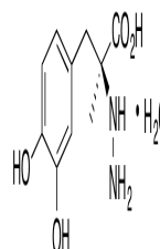
Chemical structure of S-( )-Carbidopa Monohydrate
