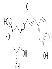
Chemical structure of Chlorogenic Acid (...)
