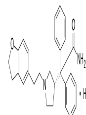
Chemical structure of Darifenacin Hydrob...
