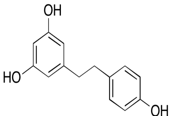
Chemical structure of , -Dihydroresveratrol
