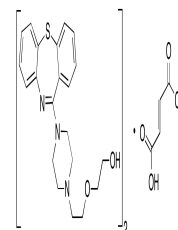
Chemical structure of Quetiapine Fumarat...
