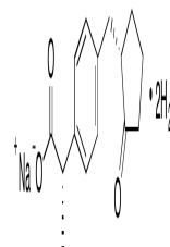
Chemical structure of Loxoprofen Sodium ...
