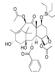
Chemical structure of 7-(Triethylsilyl)-...
