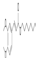
Chemical structure of n-Octyl-3
