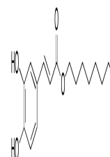
Chemical structure of n-Octyl Caffeate
