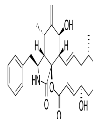
Chemical structure of Cytochalasin B
